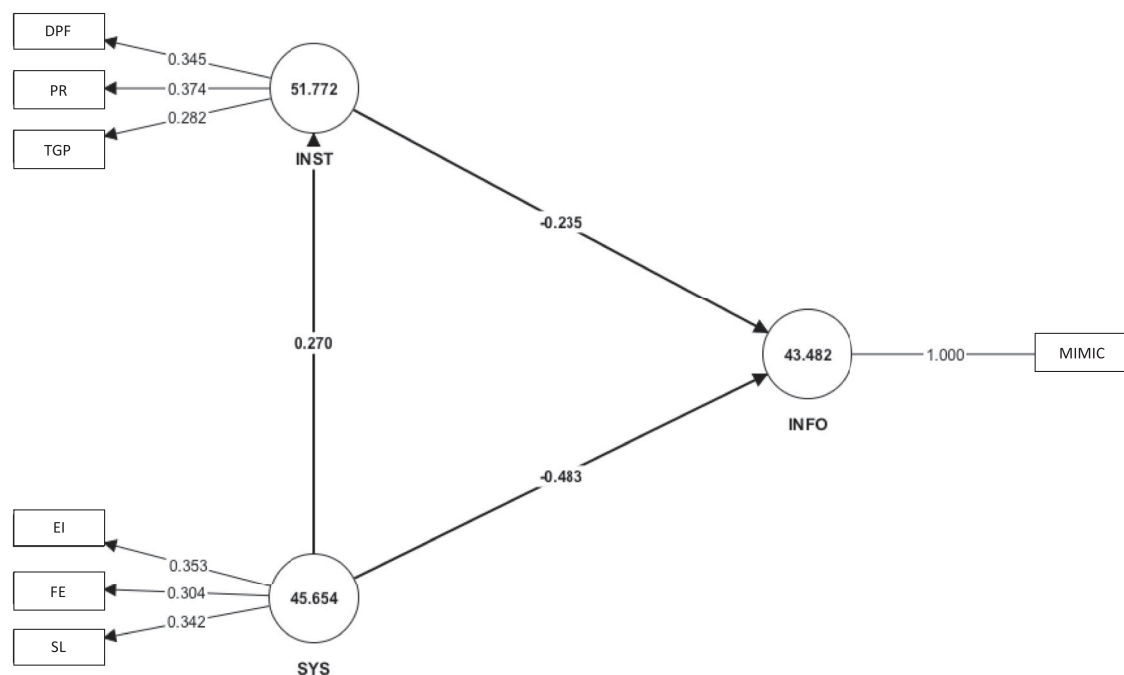
Figure 4. IPMA results complete sample. Source: Results from SmartPLS4.
