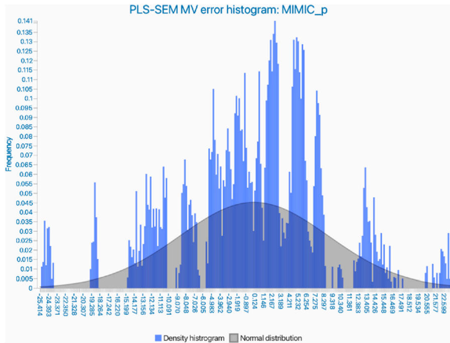
Figure 3. Prediction error distribution. Source: Results from SmartPLS4.
