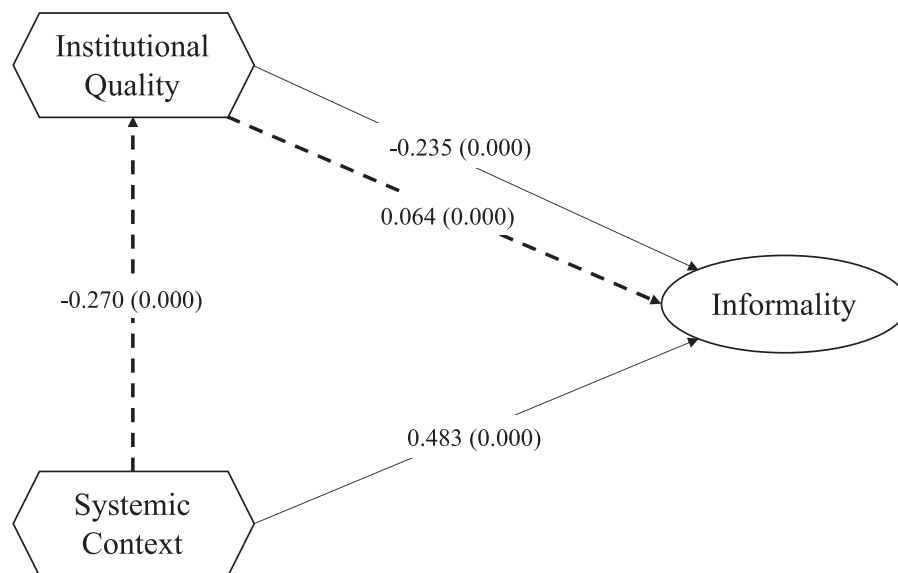
Figure 2. Model's results. Source: Authors' elaboration based on the results from SmartPLS4 – See Table 7.
