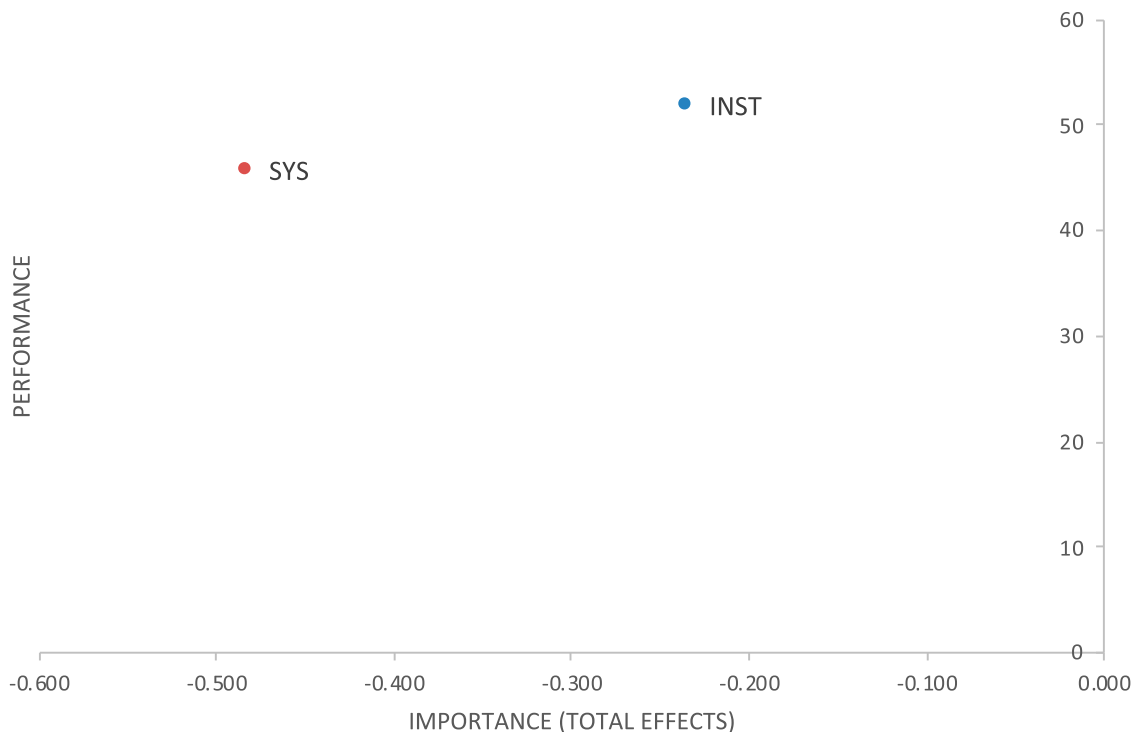
Figure 5. Importance-Performance Map. Source: Authors’ elaboration based on the results from SmartPLS4.
