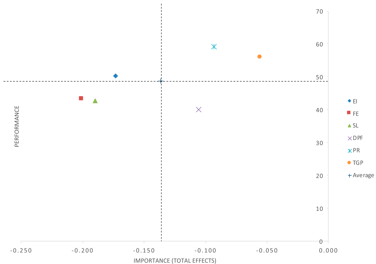
Figure 6. Indicators' Importance-Performance Map. Source: Authors' elaboration based on the results from SmartPLS4.
