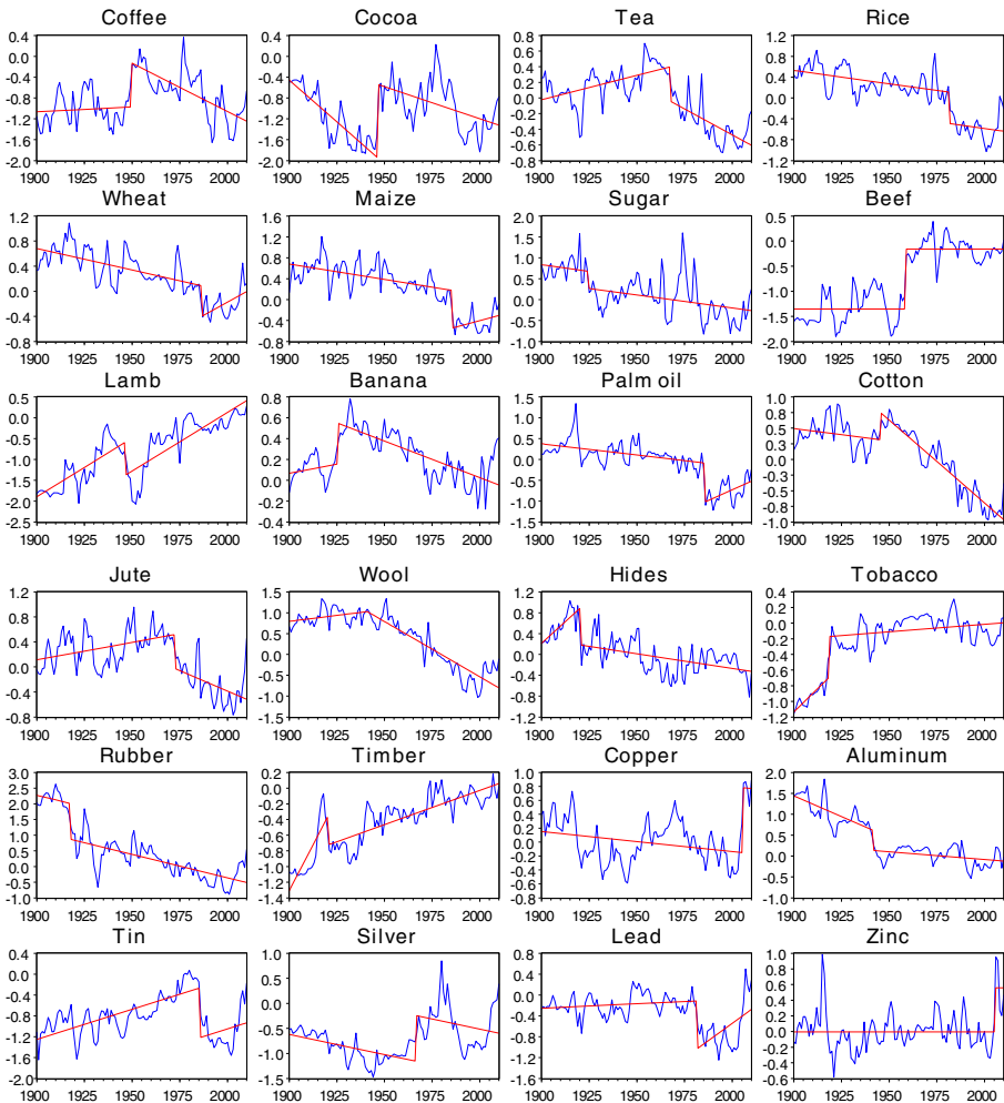
Fig. 1 Plots of the commodity price series and fitted broken trend
