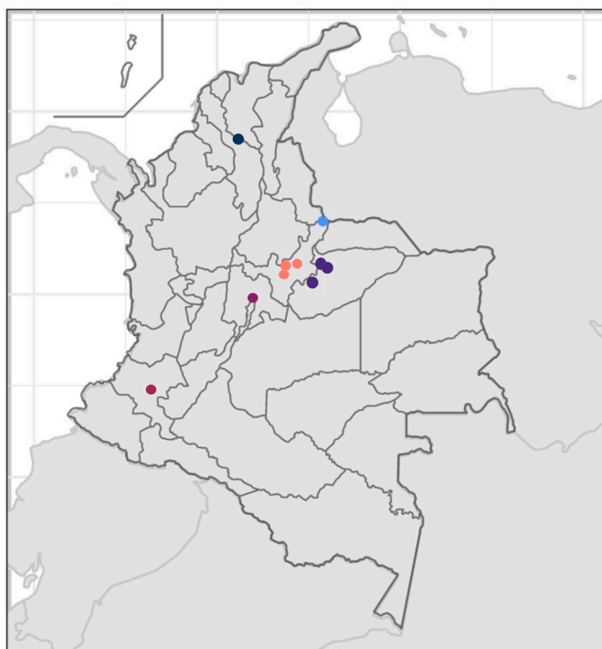
Fig. 1. Geographic Distribution of Sample Collection. Exact geographical location from the municipalities where the samples were collected are indicated in dots of distinct colors by department. The total number of samples and host from which those were taken are exhibited in the Location legend.
