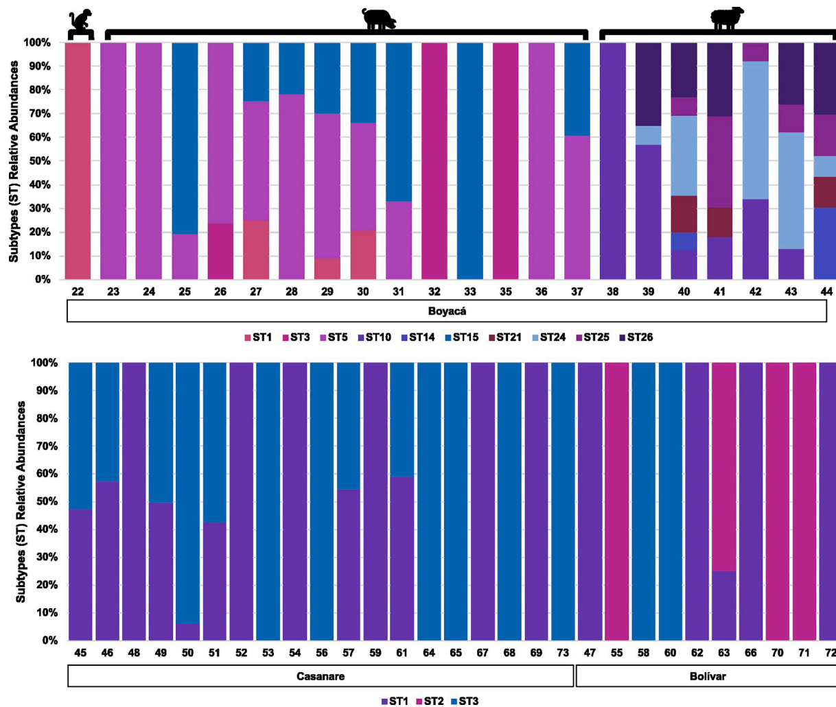
Fig. 4. Blastocystis Variation between STs in animal and human hosts. In this study was performed the detection of mixed and unique infection from different Blastocystis subtypes. Bar plots were constructed by host to reveal the percentage of each ST detected by sample. All subtypes were assigned a color to distinguish them from each other. a. Blastocystis STs diversity in animal hosts. b. Blastocystis STs diversity in humans by department.
