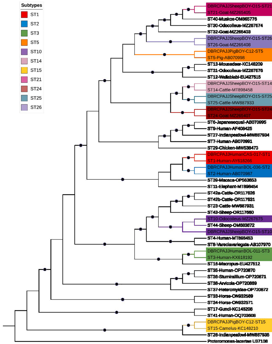
Fig. 2. Phylogenetic Relationships from the full-length SSU rRNA gene sequences obtained in the present study, Blastocystis representative reference sequences from each accepted ST, and Proteromonas lacertae as the outgroup microorganism for rooting the tree.
