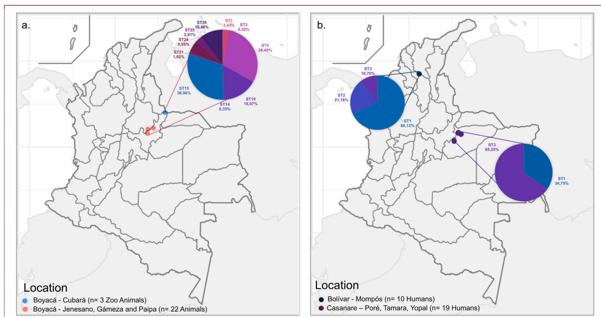
Fig. 3. Geographical Distribution of Blastocystis Subtypes in Colombia. a. Animal Samples. b. Human samples. Marked with different colored dots, the precise locations where the sequenced samples were collected are shown on the map of Colombia. Pie charts with the percentages of subtypes by department are included. The host and number of samples used for this study are specified in the legend.
